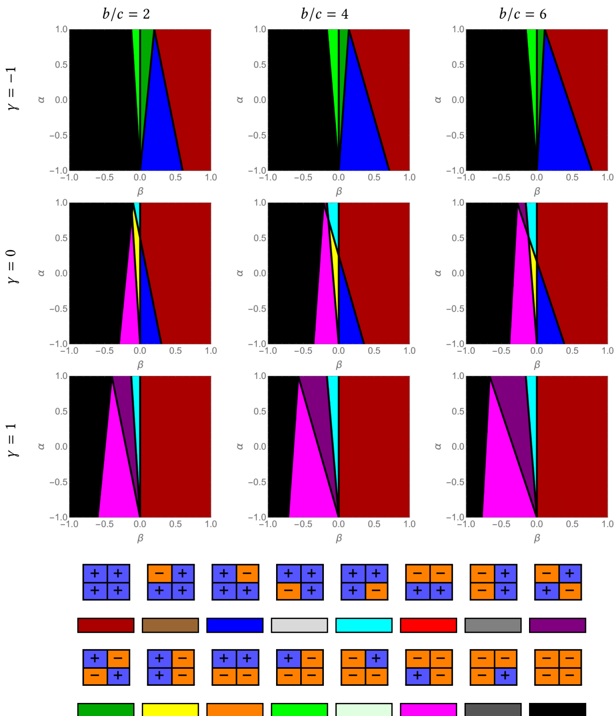
Figure B5: Phenotype space for the model where the utility depends explicitly on material payoffs (eq. 6 with k = 2 ) as a function of \beta (x-axis), \alpha (y-axis), \gamma (rows), and b/c (columns). Under the panels depicting the phenotype space, we show the color code of strategies (colors are under the corresponding utility matrix).
